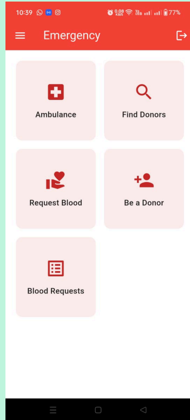
Emergency Page
