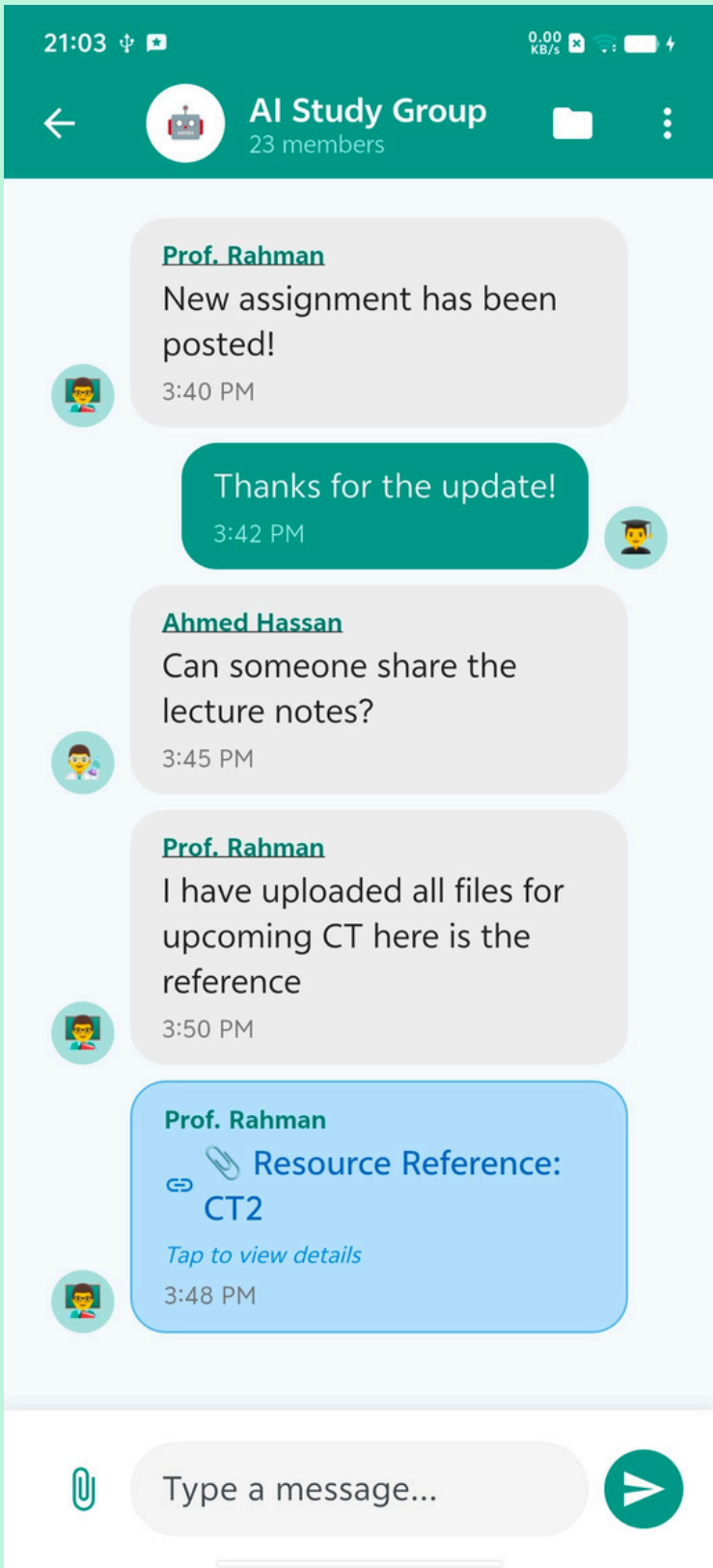
Chats View
