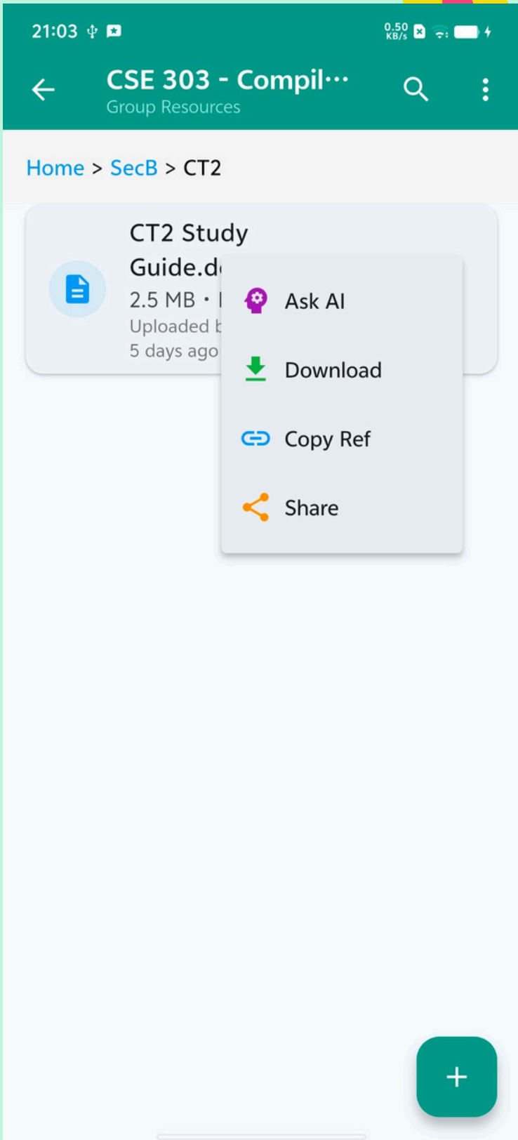
Group Resource
