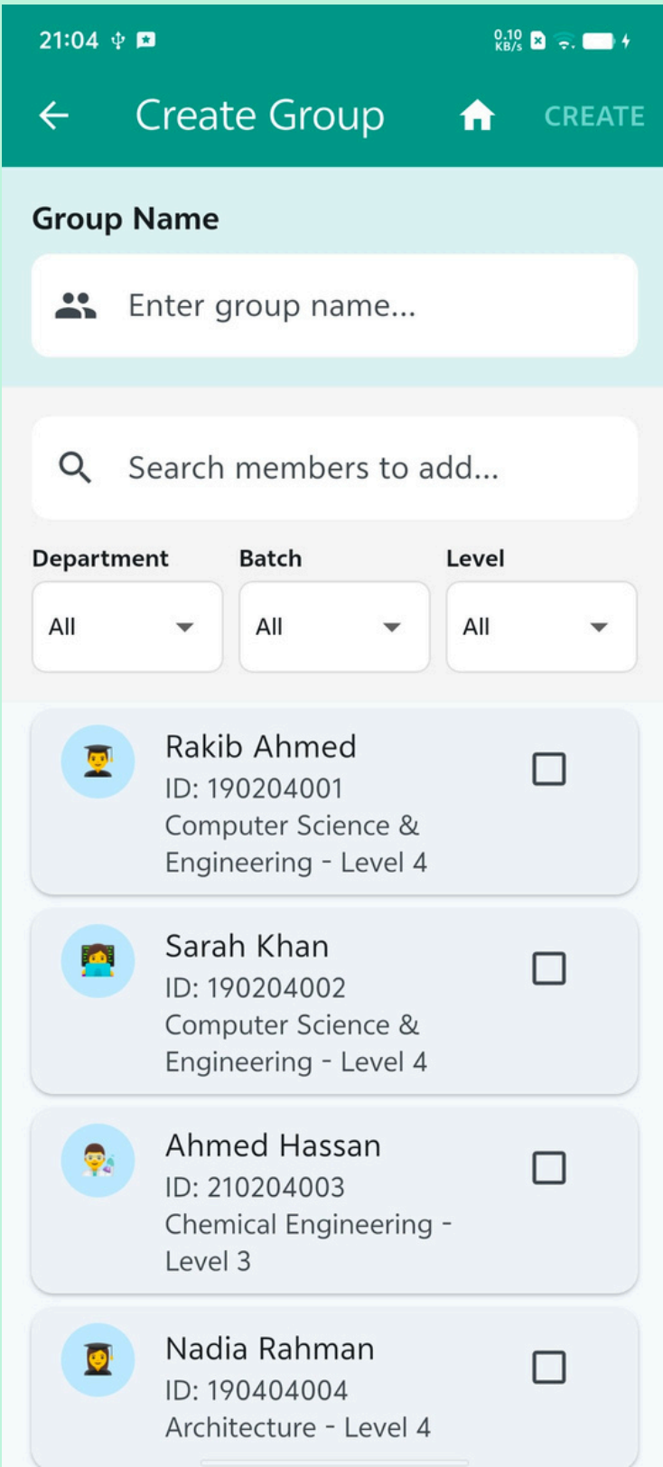
Create Chat/Group
