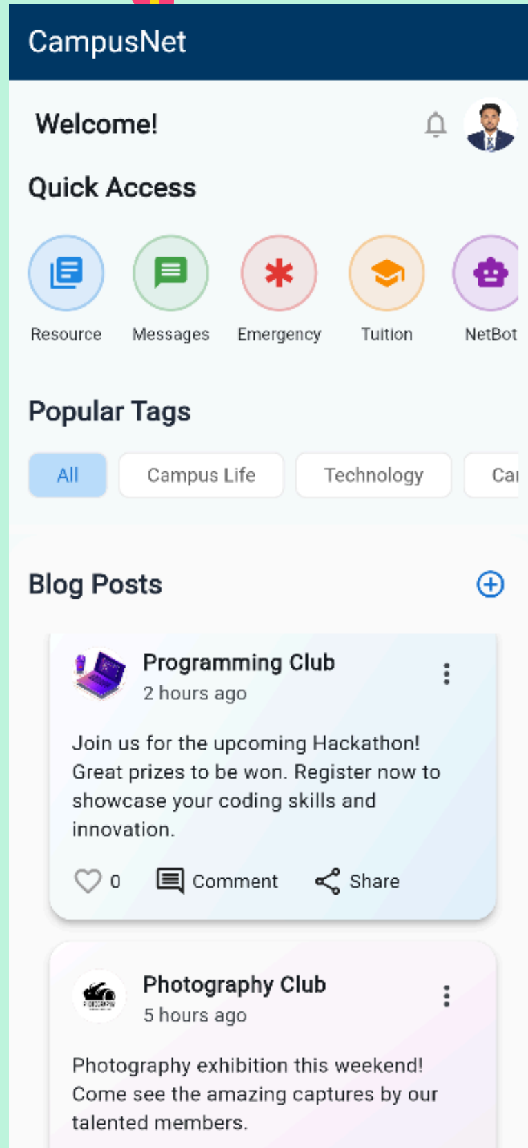
Home Page
