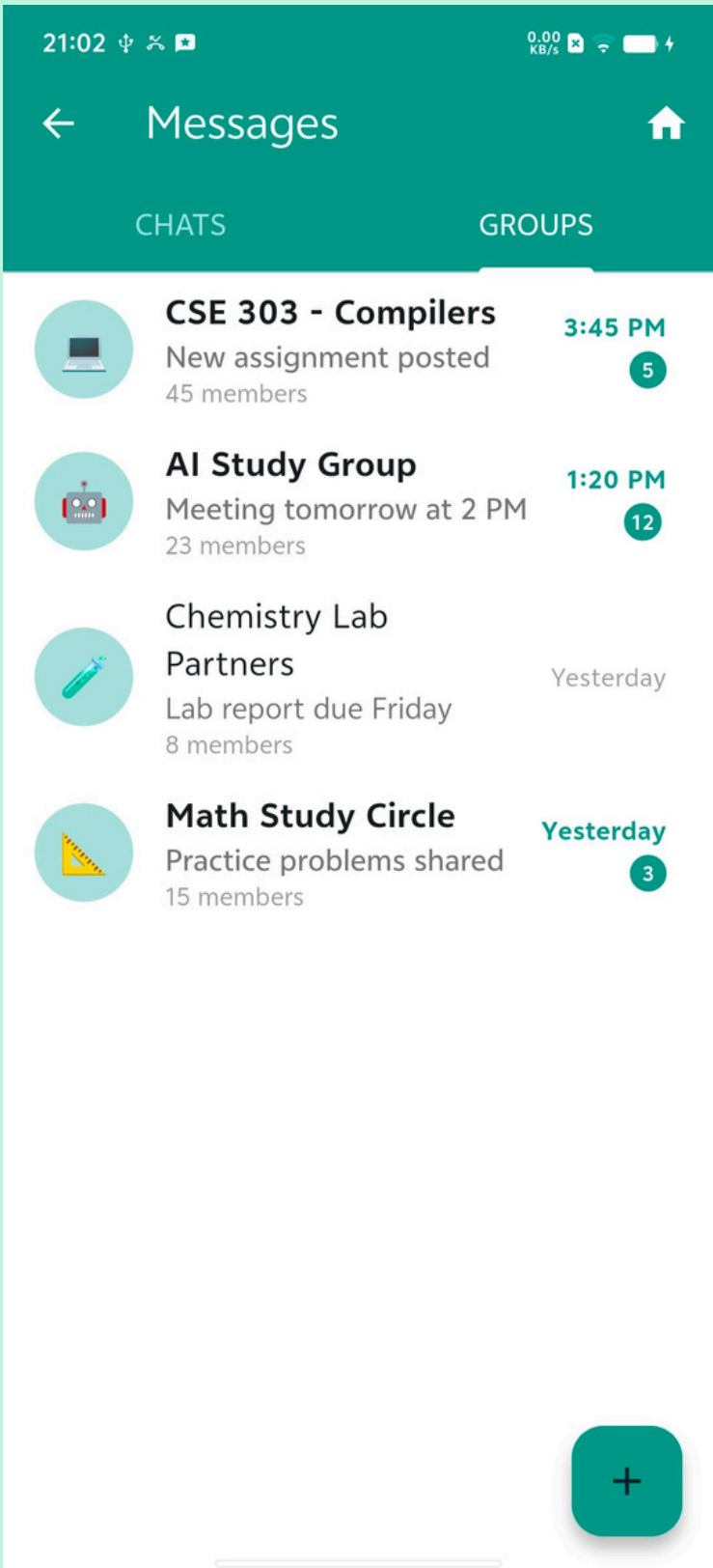
Groups
