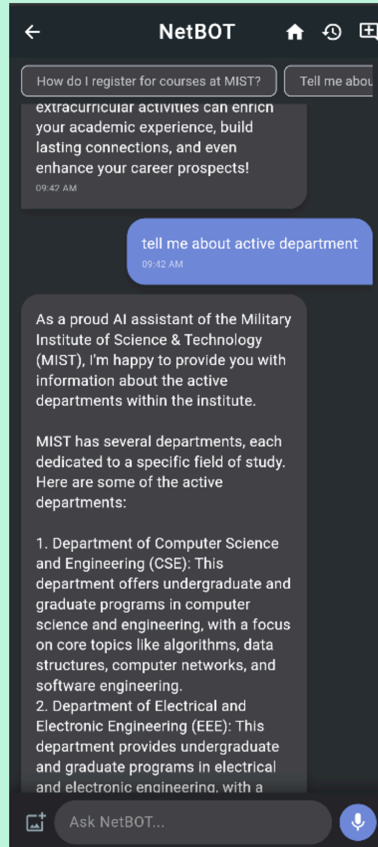
ChatBot page
