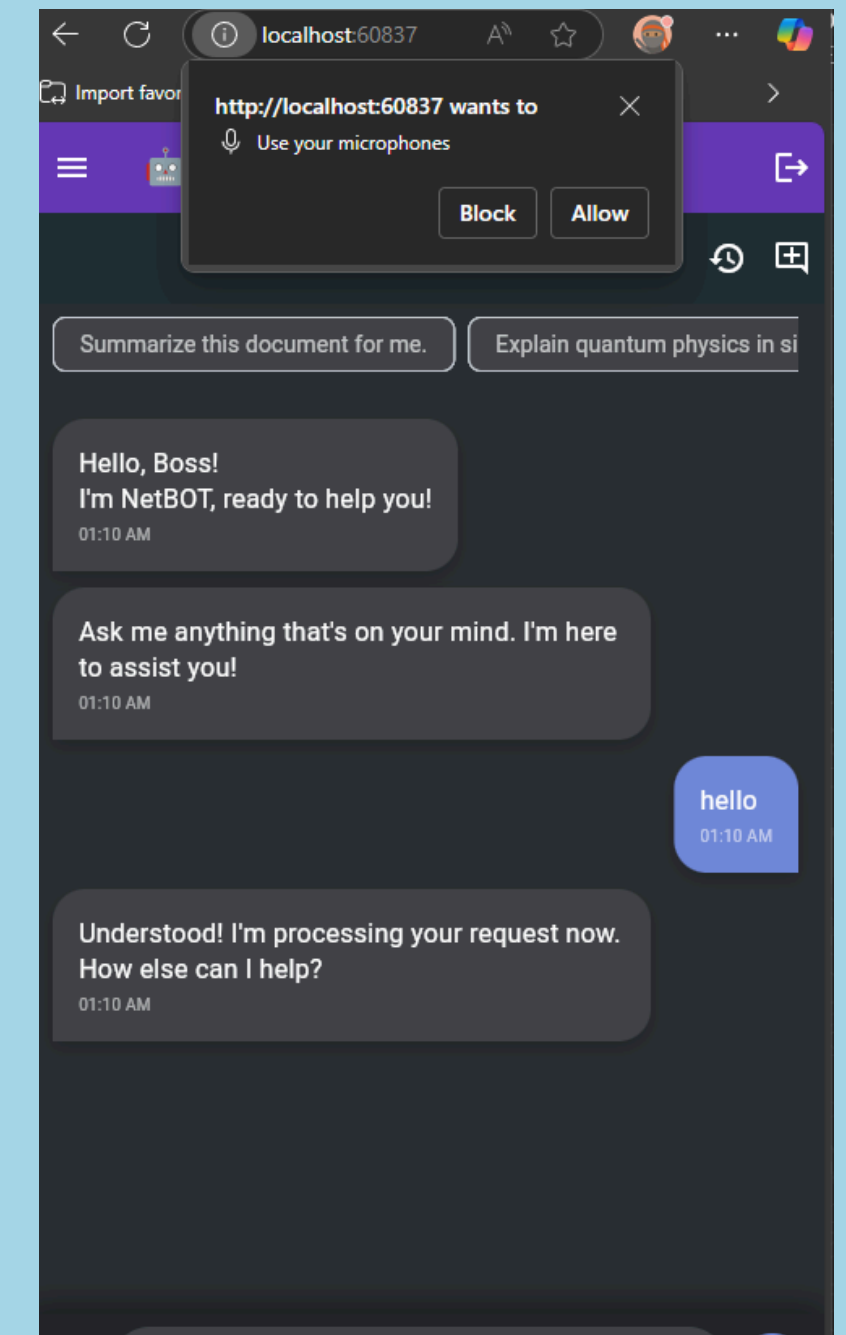
Voice Input
