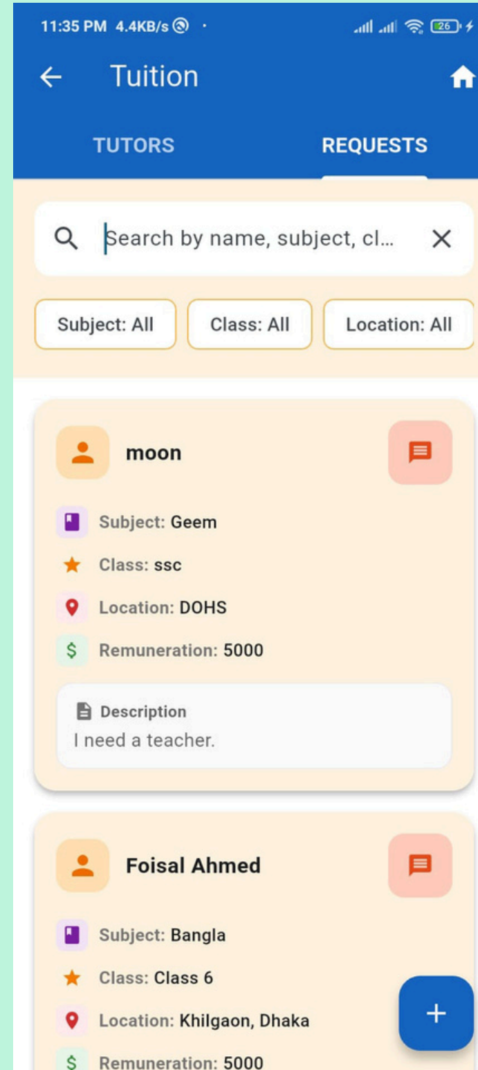
Tuition Requests
