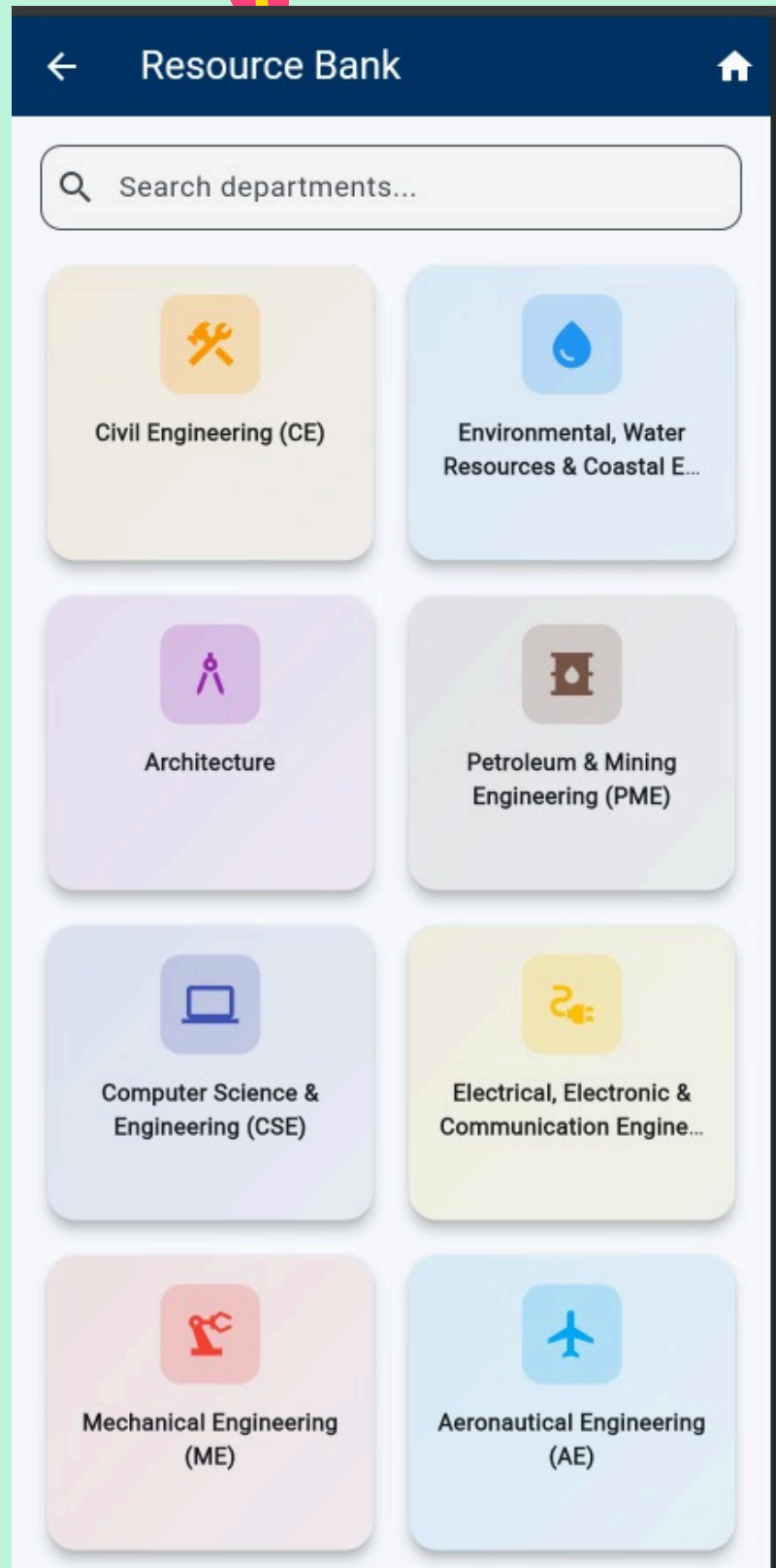
Resource Bank
